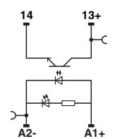
Circuit diagram
